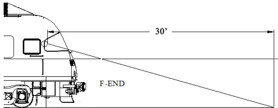
Figure 32-1: Engineer's Minimum Clear Viewing Distance from the Seated Position
