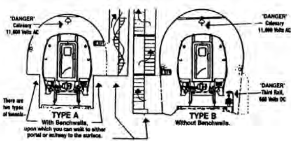
Figure 1-16 – Tunnel Hazards
