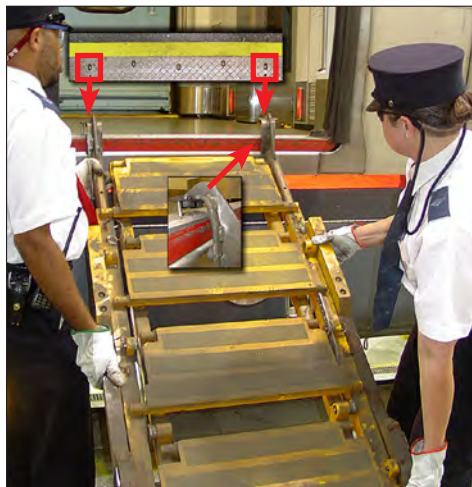
Figure 1-14 – Secure folding stairs to car body
