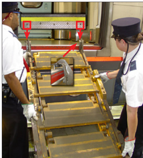
Figure 1-14 – Secure folding stairs to car body
