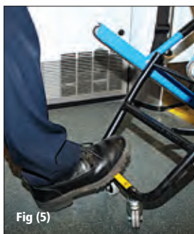
Fig (5) Align EVAC-CHAIR with top of folding stair and use foot to retract inner wheels.
